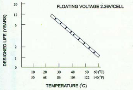
Figure 10. Accelerated Float Service Life Characteristics (DJM series )
